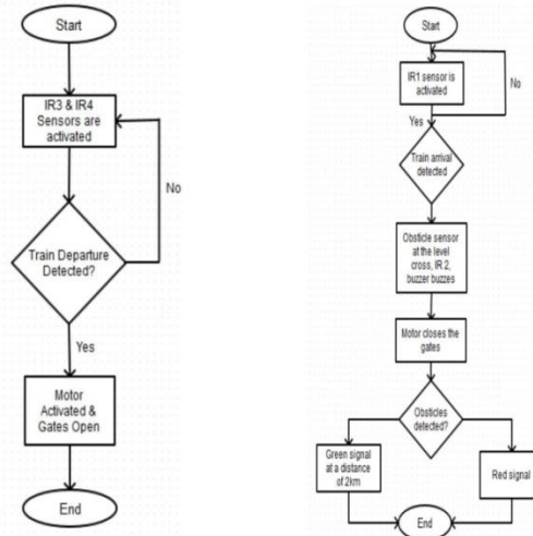
Fig.2: Architecture diagram
