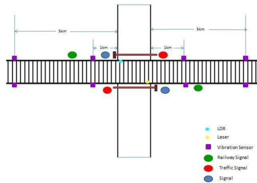
Fig. 1: Architecture diagram
