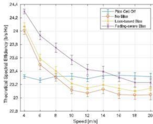
Fig. 8. Theoretical spectral efficiency as a function of the vehicular traffic speed
