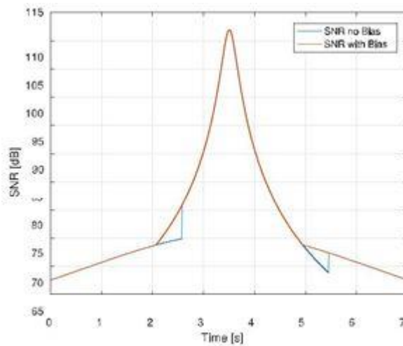
Fig. 7. \gamma^M(t) and \gamma^F(t) with a UE speed of 16 m/s. Multipath fading and shadowing are not considered in this figure for visual clarity.
