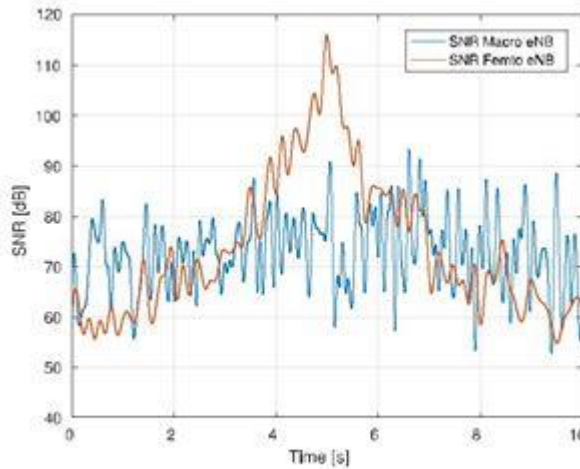
Fig. 6. \gamma_M(t) and \gamma_F(t) with a UE speed of 10 m/s. Multipath fading is not considered in this figure for visual clarity.
