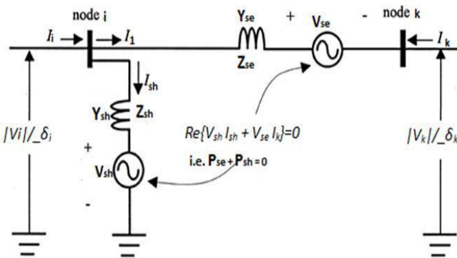
Figure 2: Equivalent circuit diagram of UPFC [25]
