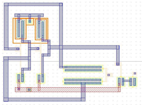
Fig 13. Layout of 9T SRAM cell
