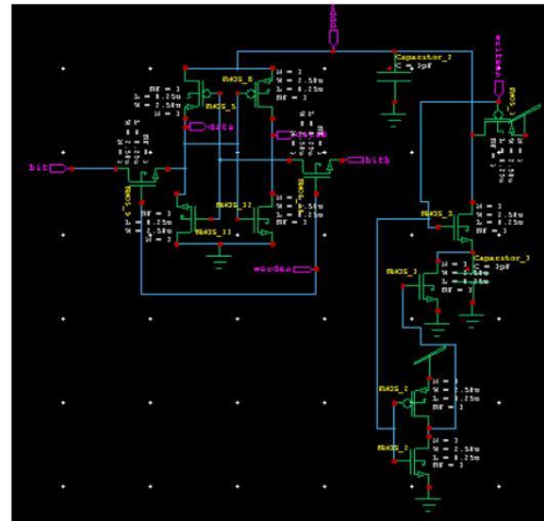
Fig. 3 capacitive LVVT circuit
