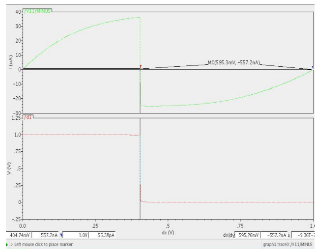
Fig. 4 Waveforms of Capacitive W-AC circuit
