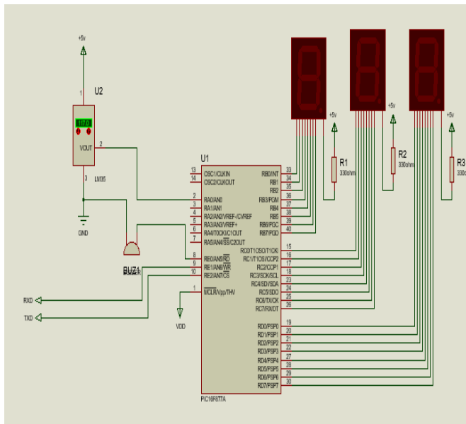
Figure: Circuit Diagram of Digital Temperature Monitoring
