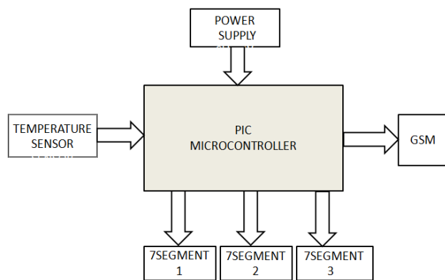
Figure: Block Diagram for Digital Temperature monitoring
