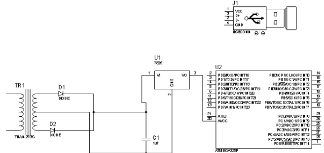
VI CIRCUIT DIAGRAM
