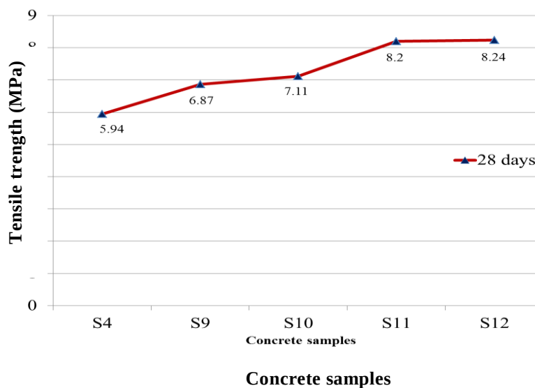
Figure 6: Comparison of tensile strength of TBC and TBFRC
