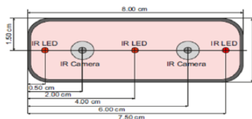
Fig. 2: Leap motion Controller
