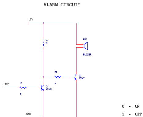
Fig-7:Alarm circuit
