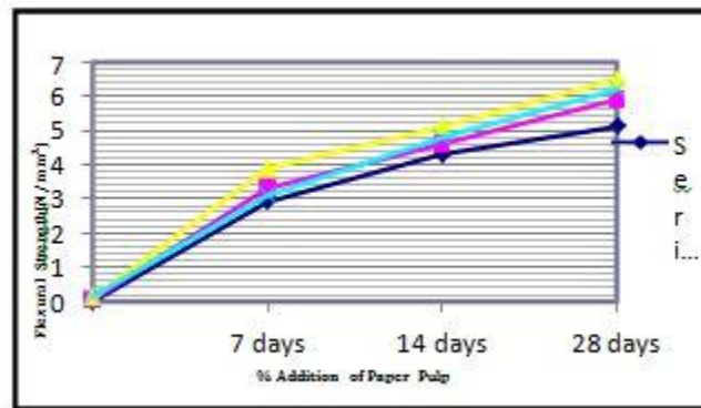
Chart -3: Flexural strength test
