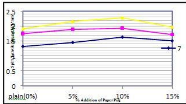
Chart -3: Split tensile strength test
