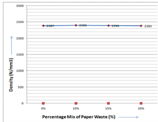
Graph 3: Variation in Density of Concrete with Different Proportions of Paper Waste at 7 days.
