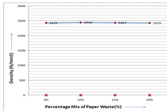
Graph 4: Variation in Density of Concrete with Different Proportions of Paper Waste at 28 days.
