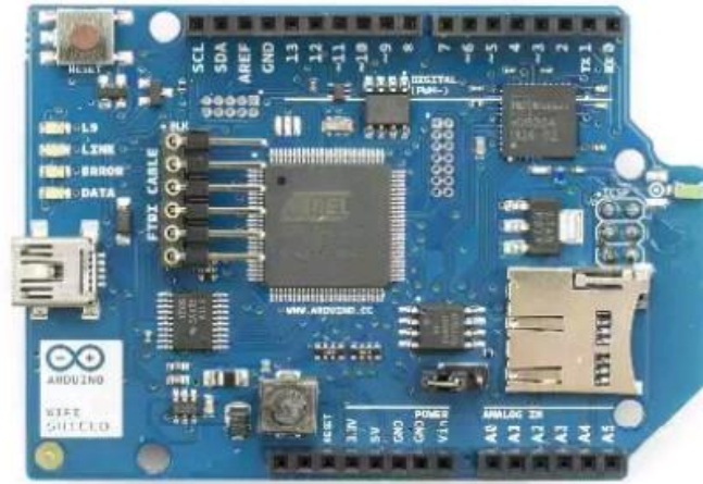
Figure 4: Arduino Wi-Fi shield
