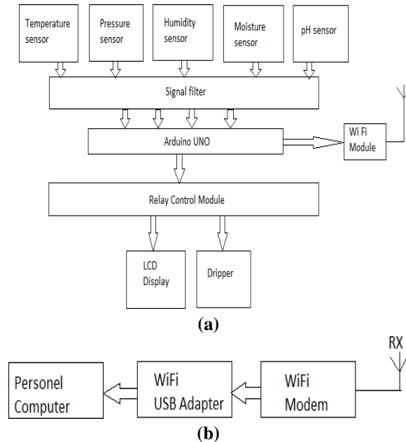
Figure 3: Block diagram of proposed model (a) Transmitter (b) Receiver
