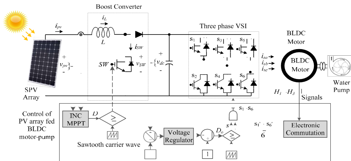
Fig.1 Configuration of PV array fed BLDC motor-pump.
