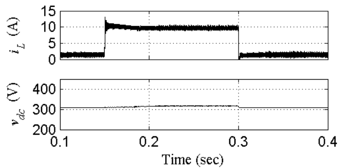
Fig.6 Dynamic performance of boost DC-DC converter
