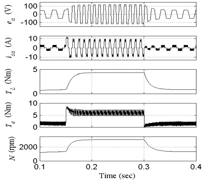
Fig.7 Dynamic performance of brushless DC motor - pump
