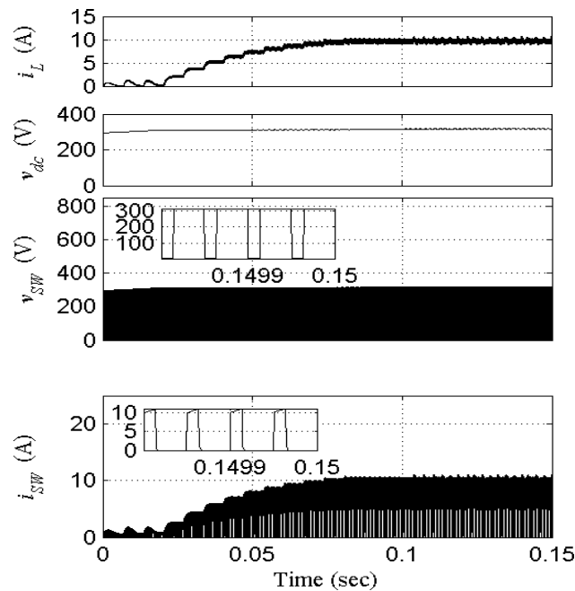
Fig.3 Starting and steady state performance of boost DC-DC converter
