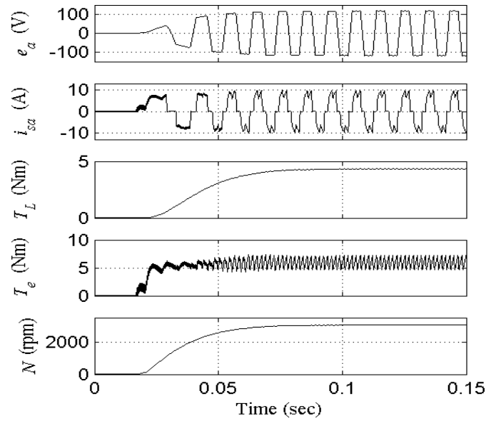
Fig.4 Starting and steady state performance of brushless DC motor-pump
