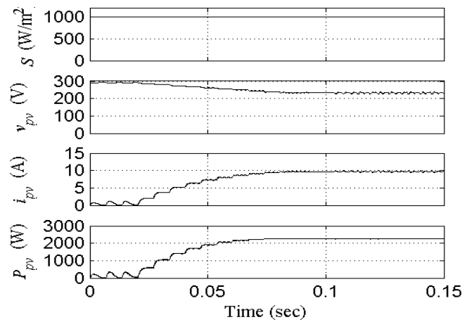
Fig.2 Starting and steady state performances of solar PV array
