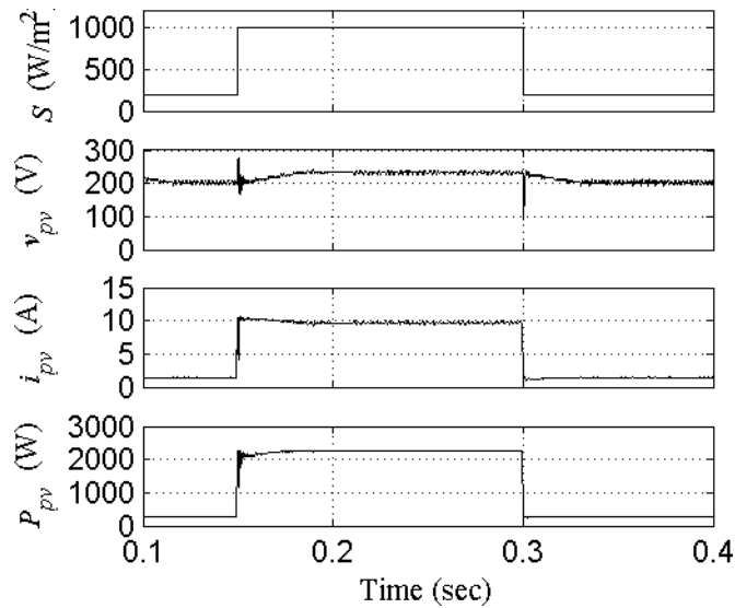
Fig.5 Dynamic performance of solar PV array
