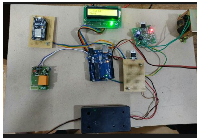
Fig. 5 experimental setup
