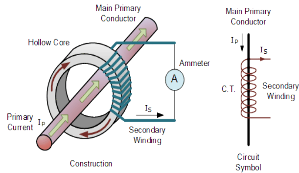
Fig [4] current transformer
