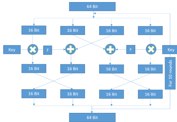
Fig. 1 Encryption Process
