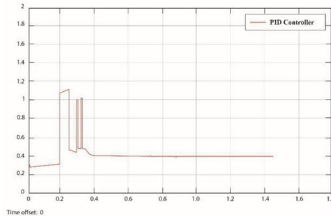
Figure 7 PID control for load restoration
