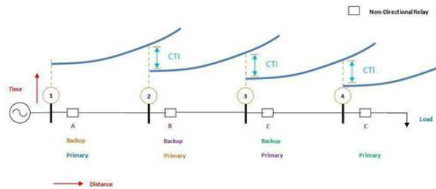
Figure 2 Coordination of DOCRs in a radial system.
