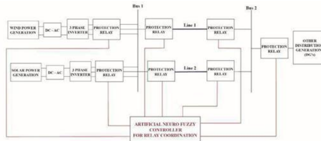
Figure 4 The Block Diagram of Proposed Methodology
