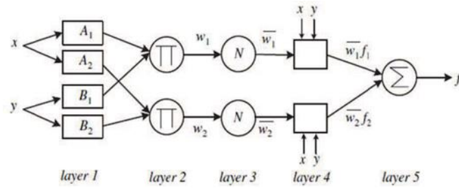
Figure 3 ANFIS architecture based on Takagi-Sugeno
