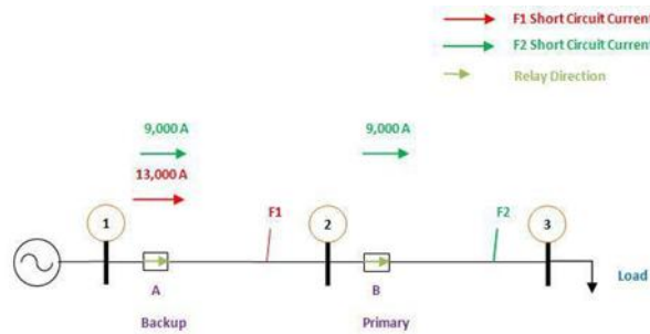
Figure 1 Indicator of fault locations: ISC
