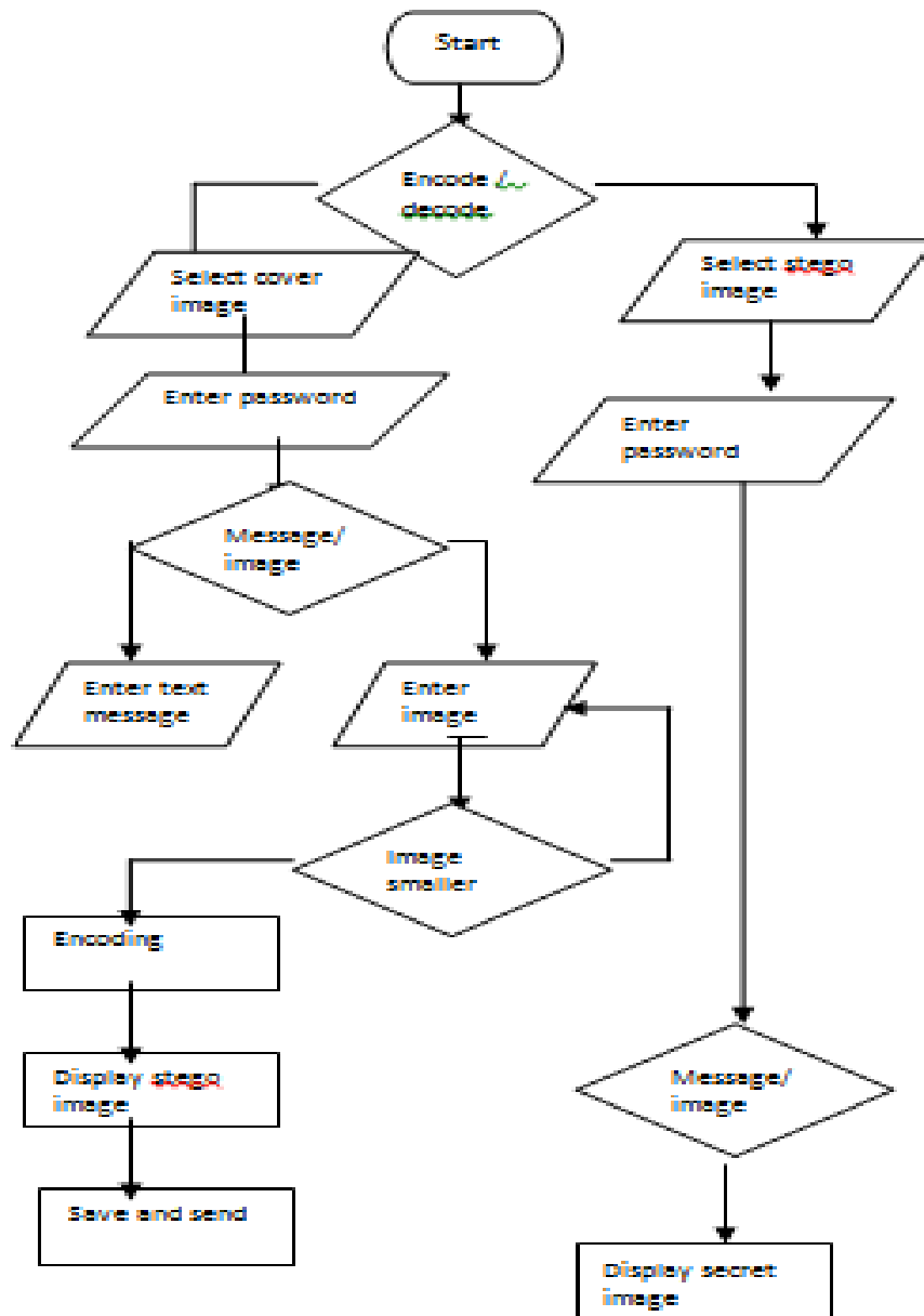
Flow chart for how the steganography apps has been works
